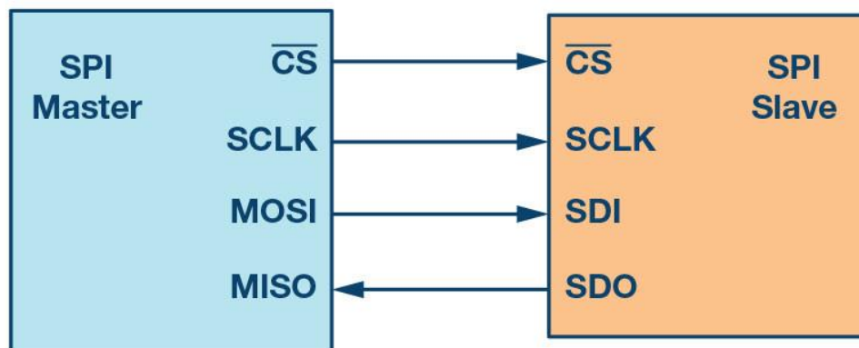
Figure 2-3: SPI configuration with master and a slave.
